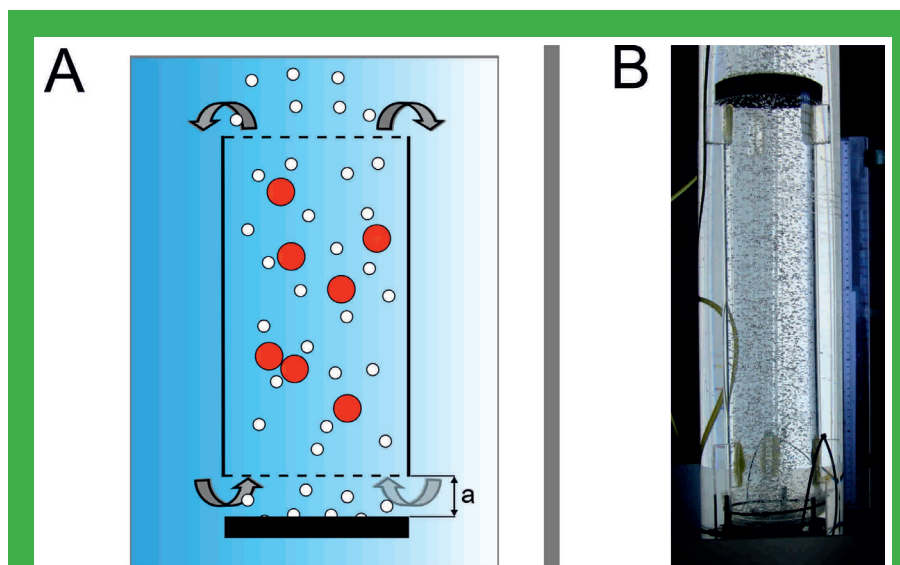
Figure 7 A: schematic view of the setup used to perform self-assembly. Air bubbles (white circles) are pumped through the diffuser that is placed under the inner tube to agitate the particles (red circles). The flow of water (the grey arrows) needed to let the particles hover is generated by the upward flow of air bubbles. We have proven that the distance a between the diffuser and the inner tube controls the flow of water into the inner tube. The
