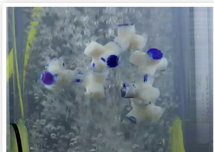
Figure 8: photograph of an experiment in which many tetrapods were entered into the system. In this case the tetrapods organize into 2 separate chains. The particles are being agitated by the flow of air bubbles in the surrounding medium.
